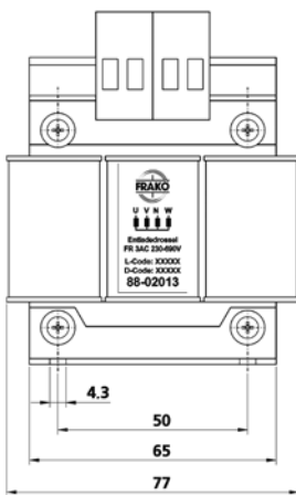
Dimensional drawing FR3AC230-690V
