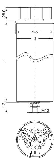
Three-phase capacitor with d = 60/70 mm
