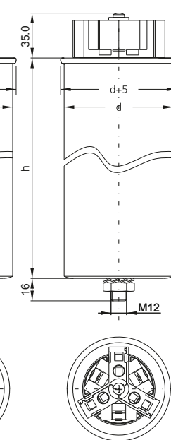
Three-phase capacitor with d = 85 mm
