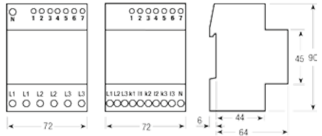
Dimensional drawing EM-EC 35, EM-EC 35 MID
