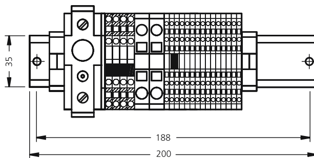
Dimensional drawing RKL-EMR 1100
