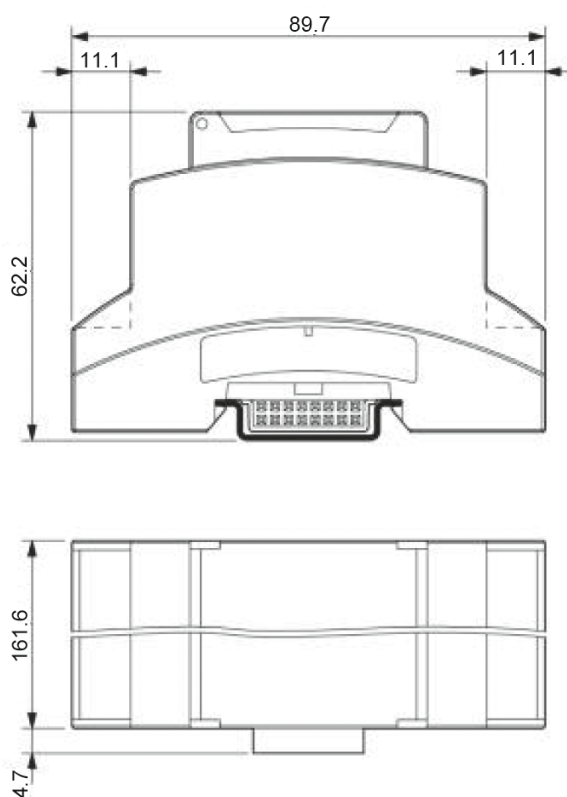
Dimensional drawing EM-PQ 2300
