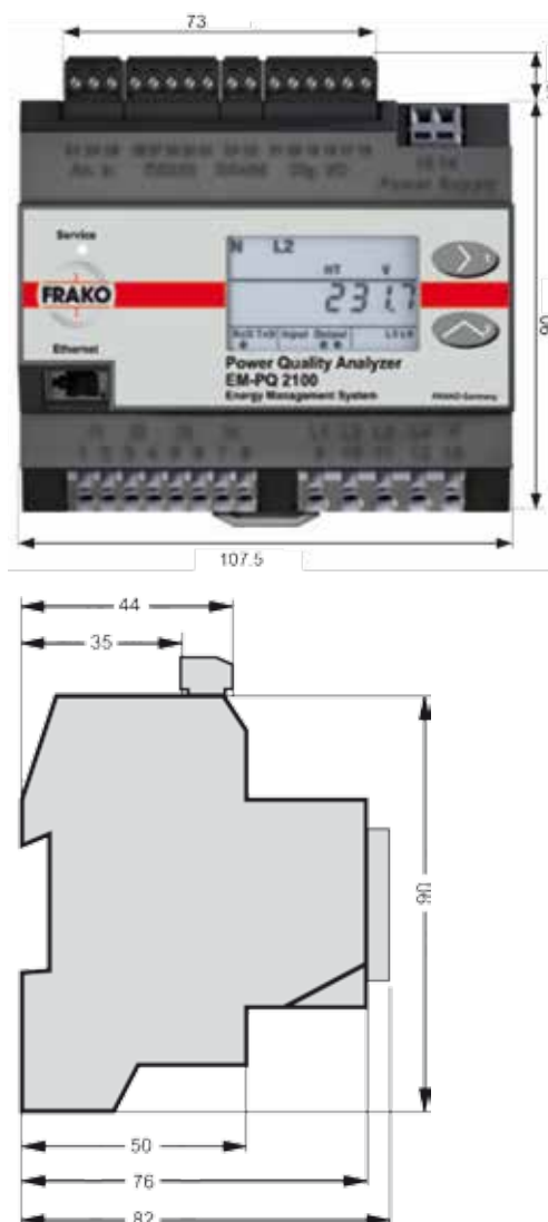
Dimensional drawing EM-PQ 2100
