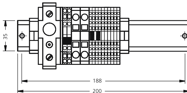
Dimensional drawing RKL-RM 9606
