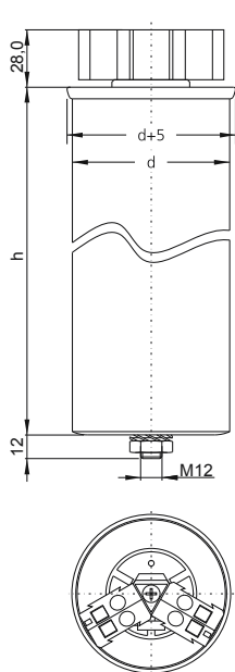
Single-phase capacitor with d = 60/70 mm
