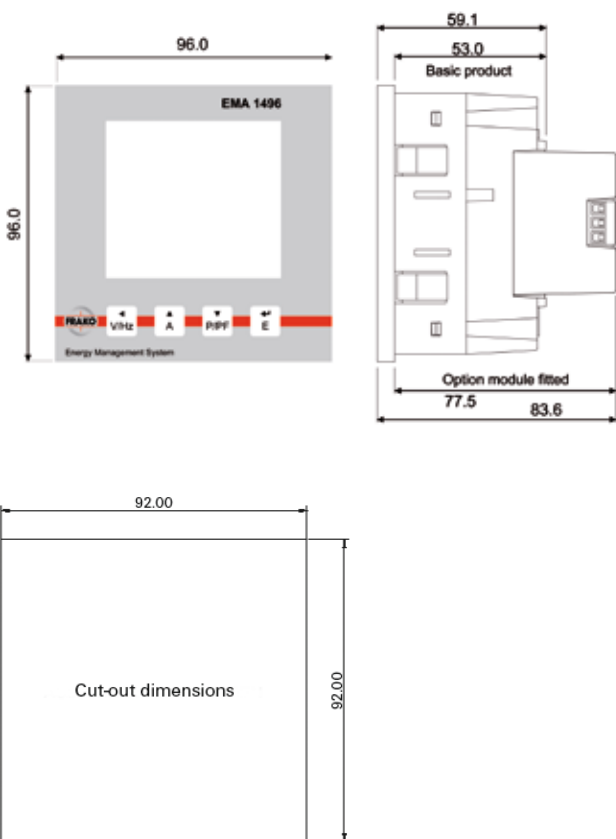
Dimensional drawing EMA 1496
