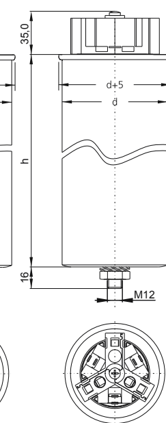
Single-phase capacitor with d = 85 mm
