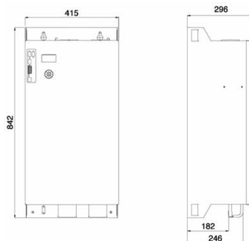
Dimensional drawing OSFD 30-415-4, OSFD 60-415-4
