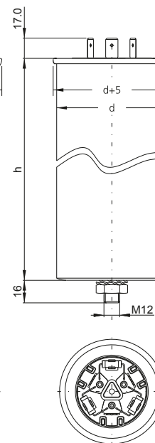
Three-phase capacitor with d = 85 mm
