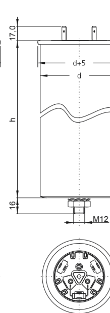
Single-phase capacitor with d = 85 mm
