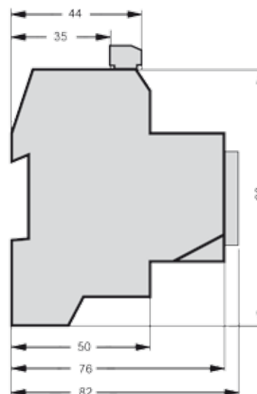
Dimensional drawing EM-PQ 2200
