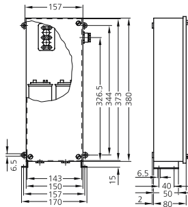
Dimensional drawing LKN Case type 1 (7.5 to 10 kvar)
